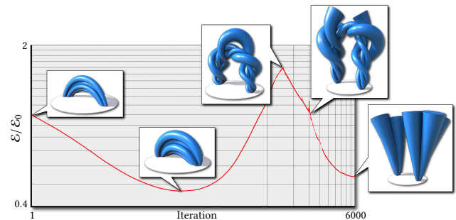
Fig. 13. Time evolution and plot of energy (16) of a twisted curve configuration over a single sunspot pair, obtained by moving the base points [Prior and Yeates 2016a,b; Rachmeler et al. 2009]. This can be viewed as a model for a coronal mass ejection: in the twisted state the energy is larger than in the final erupted state—the difference being the amount of energy ejected into space.
