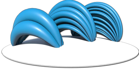
Fig. 6. A flux tube with non-circular cross-section discretized into magnetic filaments, using three different resolutions.
