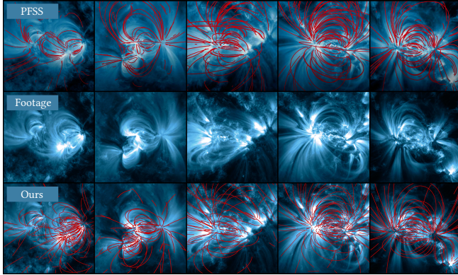
Fig. 17. PFSS field lines [Warren et al. 2018, Fig. 9] (top) compared to our magnetic filaments (bottom).
