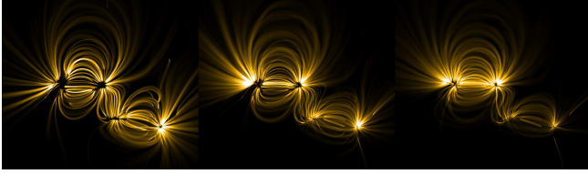
Fig. 14. Glow of an active region from Apr. 19th, 2011 computed for \rho_0 = 2 \cdot 10^{-8} (left), \rho_0 = 6 \cdot 10^{-8} (middle) and \rho_0 = 1 \cdot 10^{-7} (right). The same region was used in [Warren et al. 2018, Fig. 9] and the real footage is shown in the last column of Fig. 17.
