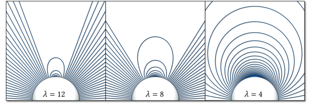
Fig. 5. The \lambda parameter controls the maximal distance 2\pi/(\lambda-2) between points on the sun that can be connected by Low geodesics.
