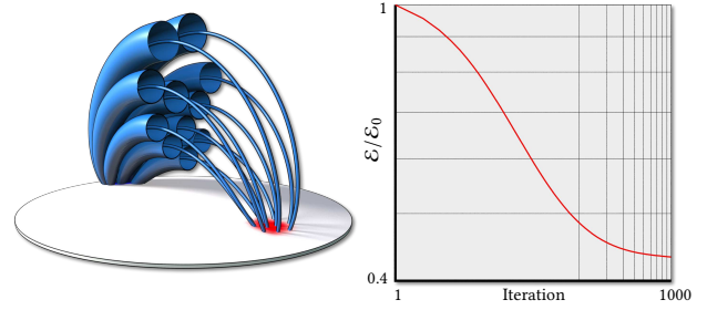
Fig. 8. The graph (right) depicts the energy \mathcal{E} relative to the initial energy \mathcal{E}_0 of the configuration as obtained by Alg. 1. The results were obtained for the example of a single sunspot pair (left).
