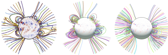
Fig. 19. The far magnetic field during the eclipse on Mar. 15th, 2015 reconstructed by the NLF-OP model (left, from [Yeates et al. 2018, Fig. 7]), the PFSS model (middle) and our model (right).
