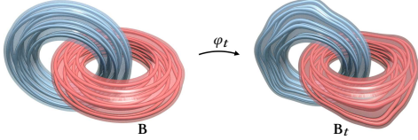
Fig. 23. A magnetic field is transported by transporting its field lines.
