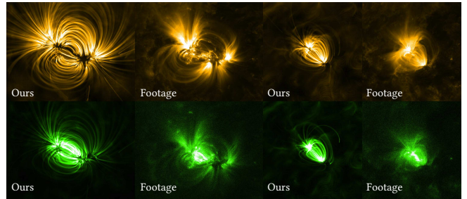
Fig. 21. Comparisons of our output to images of [NASA Solar Dynamics Observatory 2022] in extreme ultraviolet (171Å, yellow) and X-ray (94Å, green). Left half: The region studied in [Williams et al. 2020]. Right half: An active region on Jun. 19th, 2010 (compare [Warren et al. 2018, Fig. 8]).
