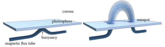
Fig. 3. Left: Below the sun's surface, a strong magnetic field is structured into a bundle of filaments by the convection flow. Right: Buoyancy makes some of these fibers rise above the sun's surface. This is the origin of the fibered structure of the corona.
