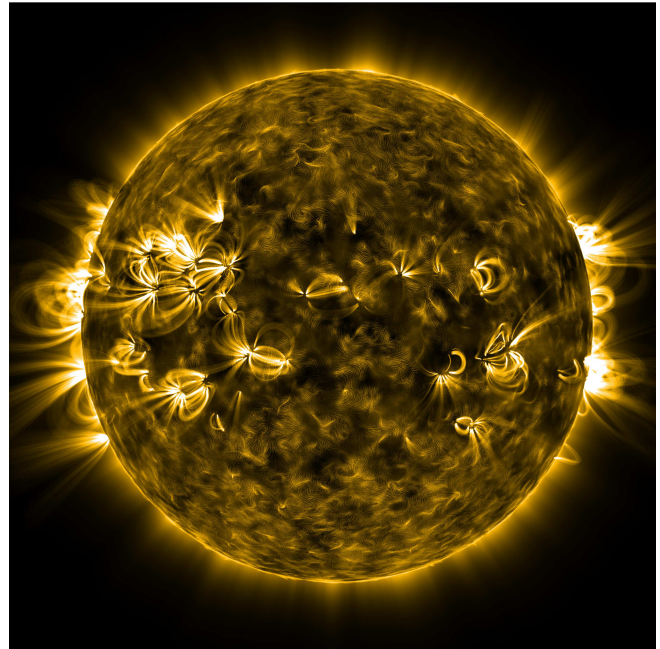
Fig. 1. A procedurally generated solar atmosphere computed by our algorithm. The underlying magnetic flux map was randomly generated and is shown in the inset on this page.
