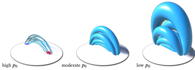
Fig. 7. For the same flux map featuring two isolated sun spots of opposite polarity, we show our computed plasma configurations for different values of the pressure parameter p_0 .
