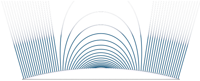
Fig. 4. Unobstructed magnetic filaments follow shortest curves in a certain metric (12). In our solar atmosphere the metric is given by (11) with \lambda = 23 . Two points whose spherical distance exceeds 2\pi/(\lambda-2) are connected by a straight path going out to infinity and back.
