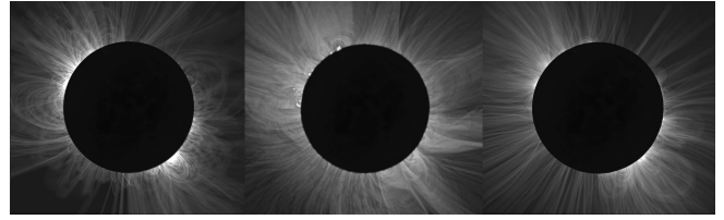
Fig. 20. The far magnetic field (middle, Image by Miroslav Druckmüller, Shadia Habbal, Peter Aniol, Pavel Štarha) during the eclipse on Mar. 15th, 2015 reconstructed and rendered by our model (right) and the PFSS model (left).
