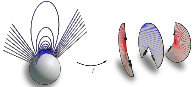
Fig. 24. The map f from Eq. (17) which maps geodesics contained in a plane on the sun's exterior to geodesics in a multiple cover of the unit disc in \mathbb{R}^2 .
