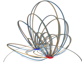
Fig. 15. If the magnetic field is so strong that we can assume p = 0 , the soul curves of magnetic filaments (blue) computed by our method are close to field lines (yellow) of a PFSS field.
