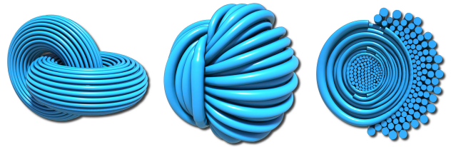
Fig. 16. A pair of linked flux tori (left) relaxed within a constant ambient gas pressure (middle, right).
