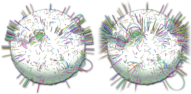
Fig. 10. Left: A curve configuration initialized from the stippling in Fig. 9 of the flux map of Oct. 21st, 2011. All filaments are vertical plane curves or radial straight line segments. Right: The same configuration in a relaxed state.
