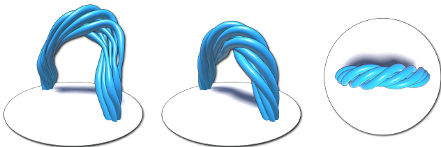
Fig. 11. An artistically prescribed collection of initial filaments with 540^\circ twist (left) and the corresponding energy minimizer (middle, right).
