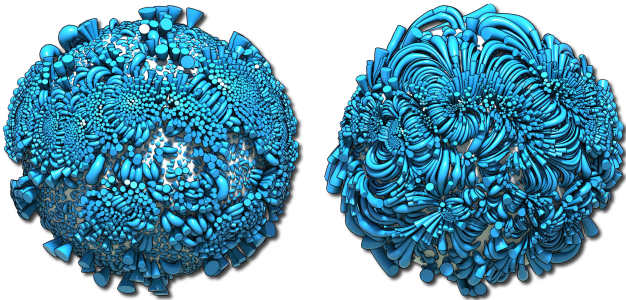
Fig. 18. Magnetic field of Oct. 21st, 2011 computed by our method (left) and PFSS (right), both visualized by magnetic filaments.
