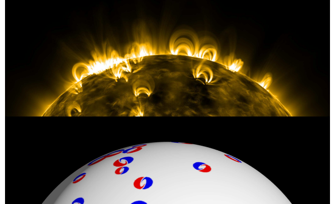
Fig. 2. An artistically designed flux map (bottom) and the corresponding solar atmosphere (top). An animated version is provided in the supplementary material.
