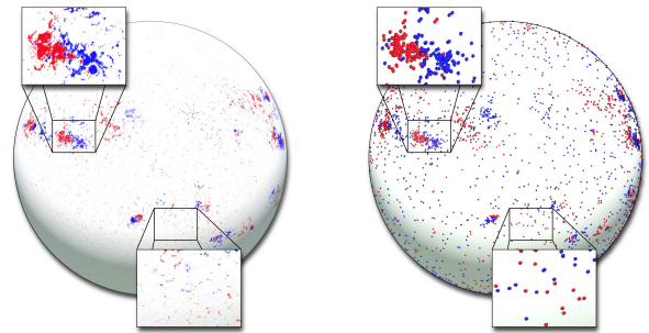
Fig. 9. A stippling (right) of the flux density map from Oct. 21st, 2011 (left).
