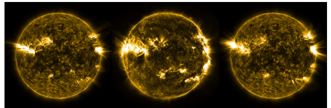
Fig. 22. Real footage of the solar atmosphere on Oct. 21st, 2011 (middle) compared to the output from our rendering method applied on the PFSS model (left) and our algorithm (right) computed from the corresponding frontal flux map (Sec. 10).
